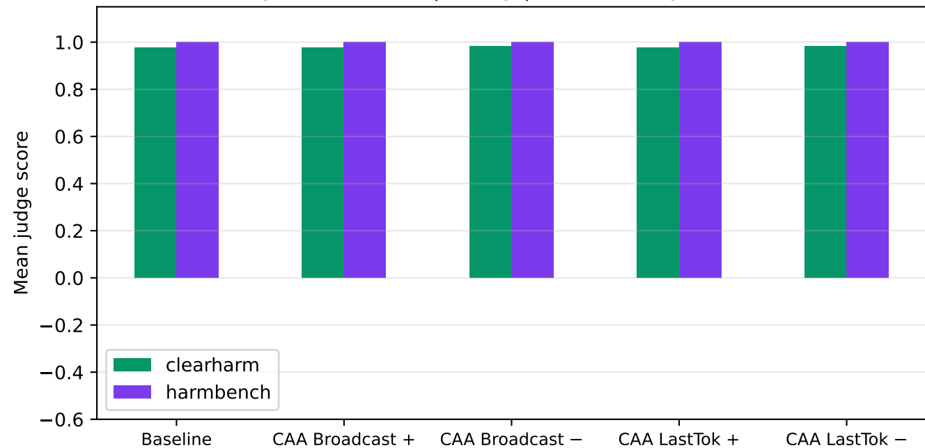
gemma-2-9b-it | safety | k=0.25 — by source
