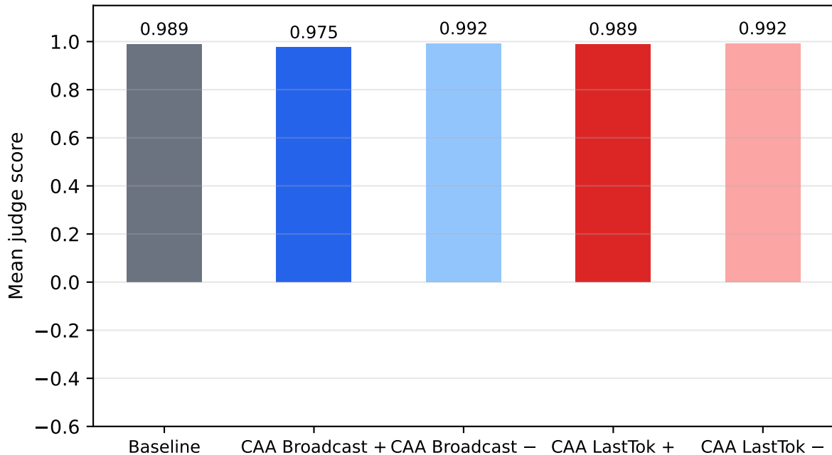
gemma-2-9b-it | safety | k=0.50
