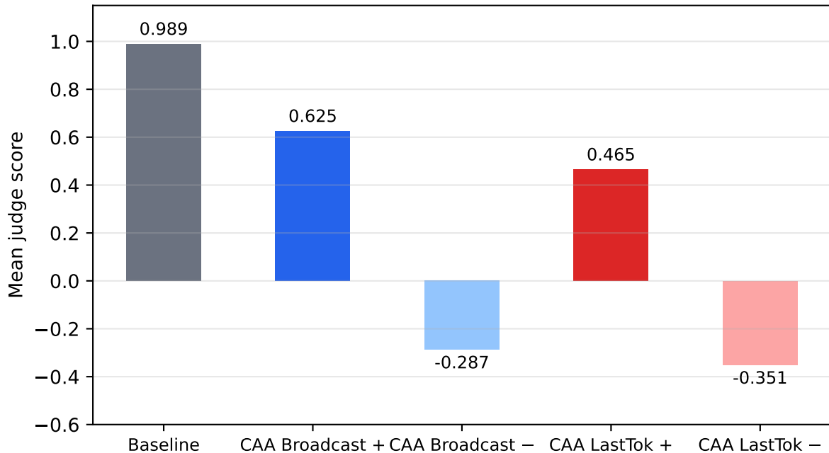
gemma-2-9b-it | safety | k=3.00
