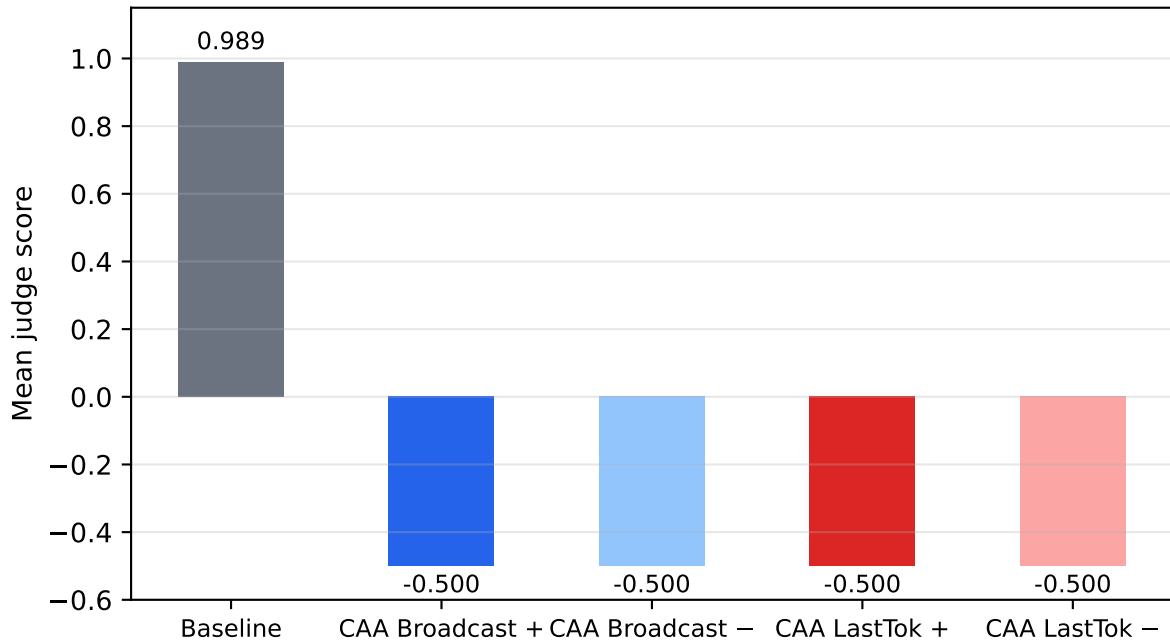
gemma-2-9b-it | safety | k=5.00
