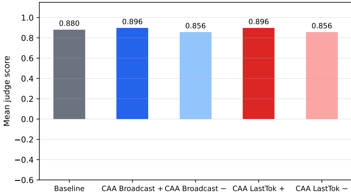
llama-3.1-8b-instruct | safety | k=0.25
