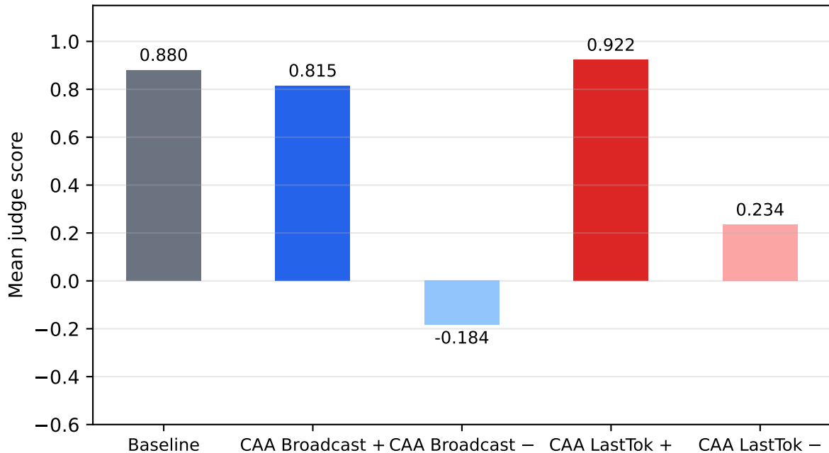
llama-3.1-8b-instruct | safety | k=3.00
