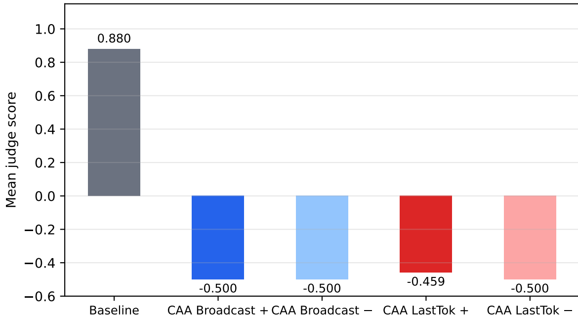
llama-3.1-8b-instruct | safety | k=5.00
