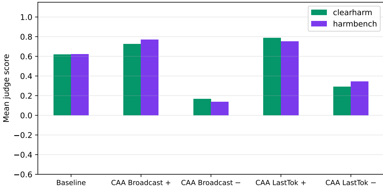
mistral-7b-instruct | safety | k=2.00 — by source
