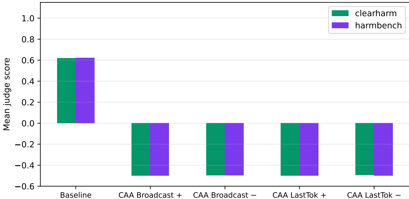
mistral-7b-instruct | safety | k=5.00 — by source
