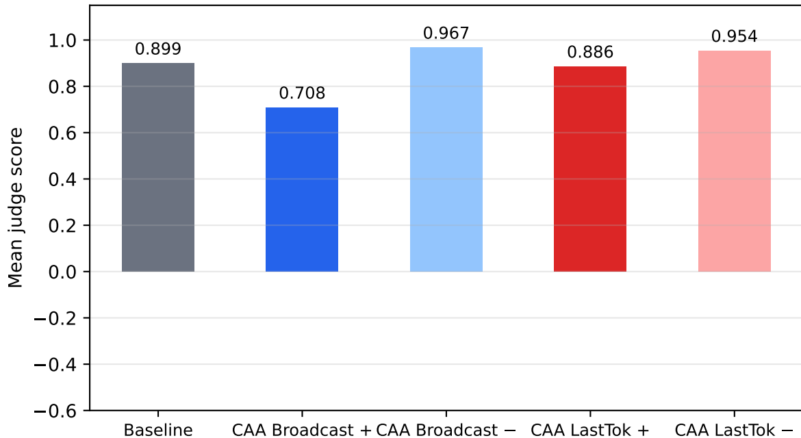
qwen2.5-7b-instruct | safety | k=1.00
