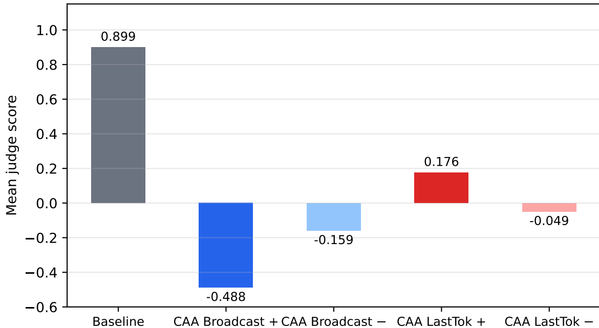
qwen2.5-7b-instruct | safety | k=2.00
