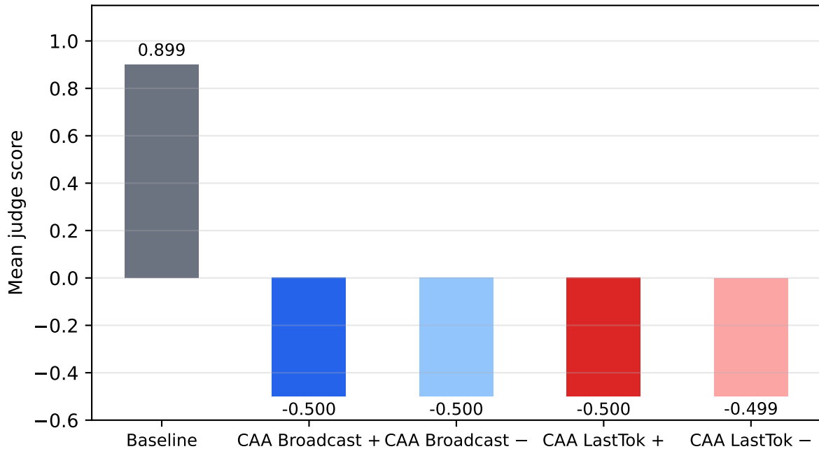
qwen2.5-7b-instruct | safety | k=3.00
