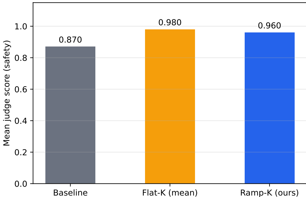
llama-3.1-8b-instruct — Flat-K vs Ramp-K
