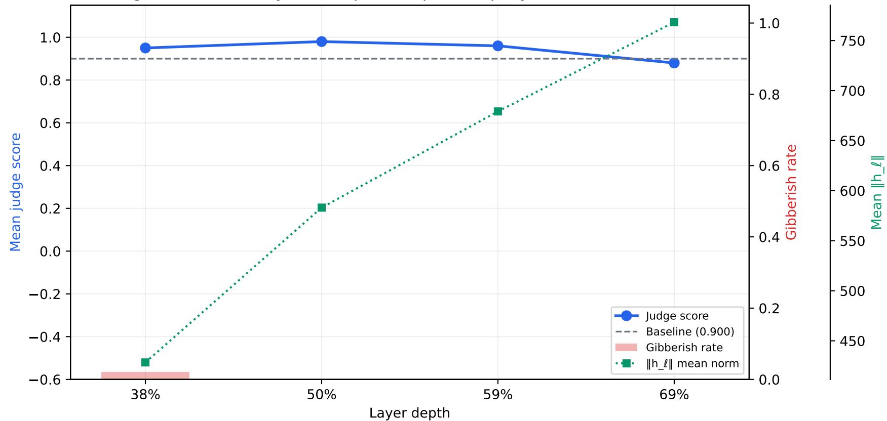
gemma-2-9b-it — Single-layer steering at K = 10 \times K_\ell High K at shallow layers collapses output; deep layers remain unsteered
