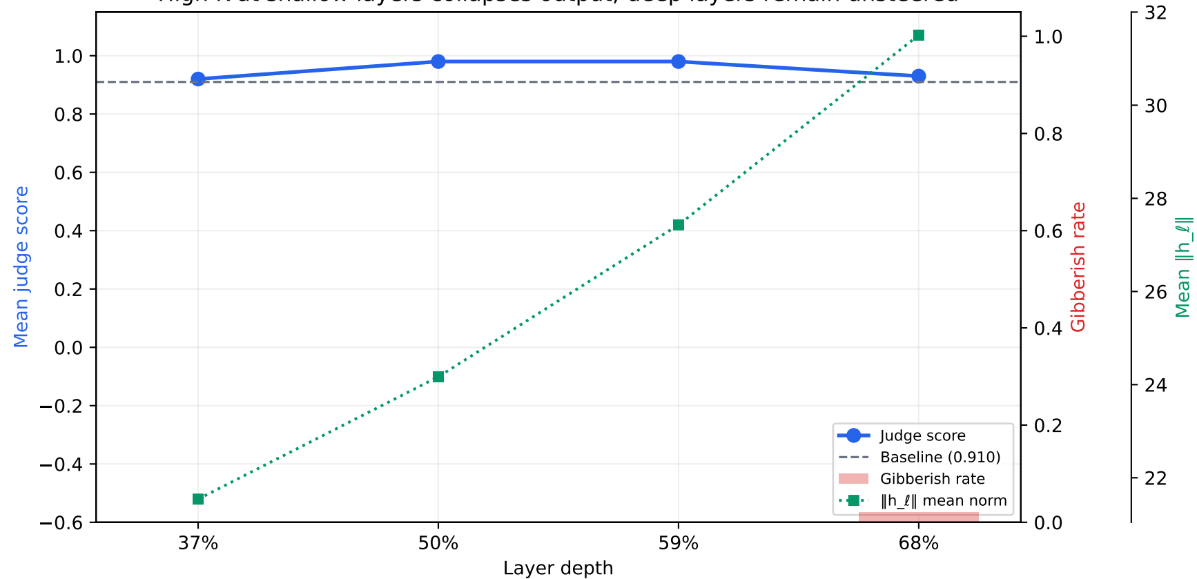
llama-3.1-8b-instruct — Single-layer steering at K = 10 \times K_\ell High K at shallow layers collapses output; deep layers remain unsteered
