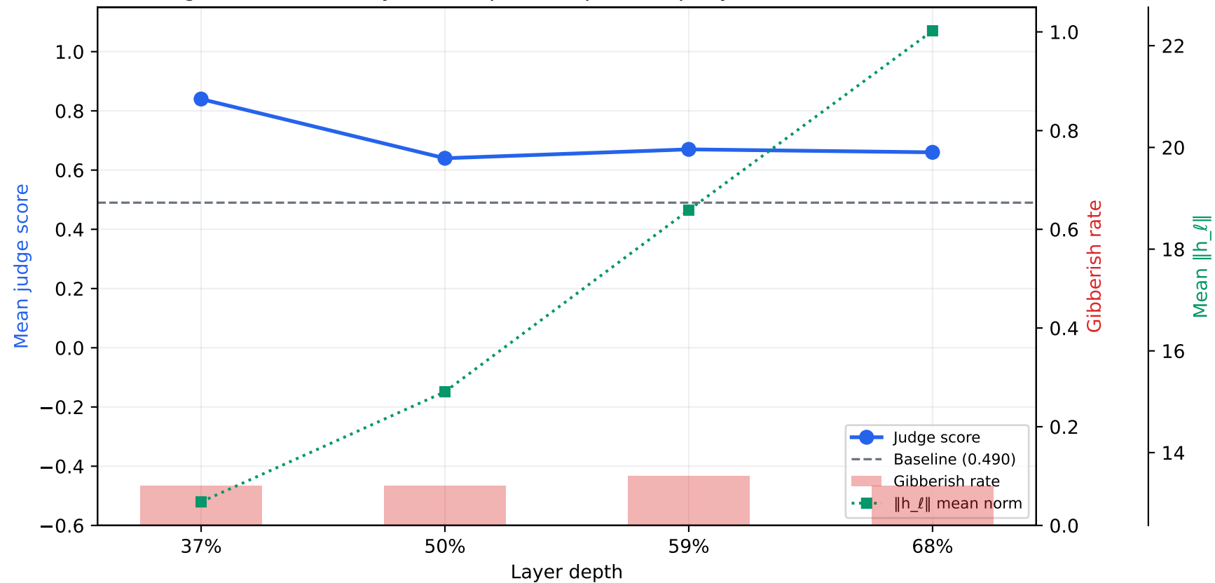
mistral-7b-instruct — Single-layer steering at K = 10 \times K_\ell High K at shallow layers collapses output; deep layers remain unsteered
