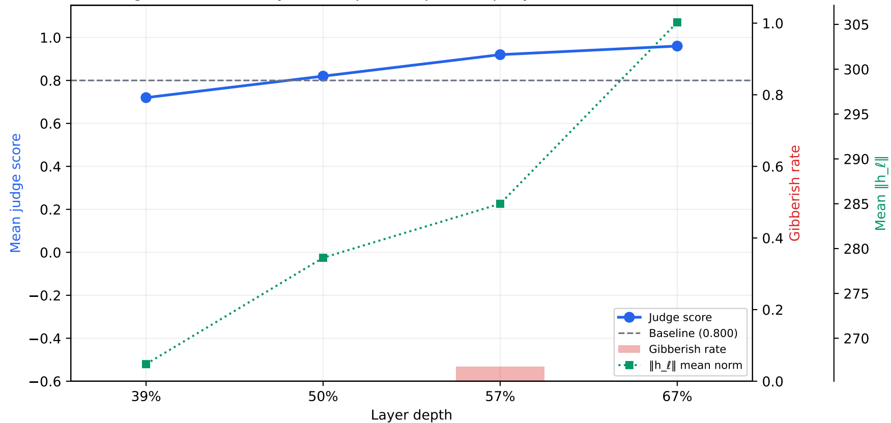
qwen2.5-7b-instruct — Single-layer steering at K = 10 \times K_\ell High K at shallow layers collapses output; deep layers remain unsteered
