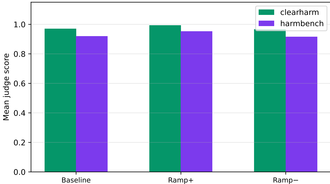
gemma-2-9b-it | safety | k=0.25 — by source
