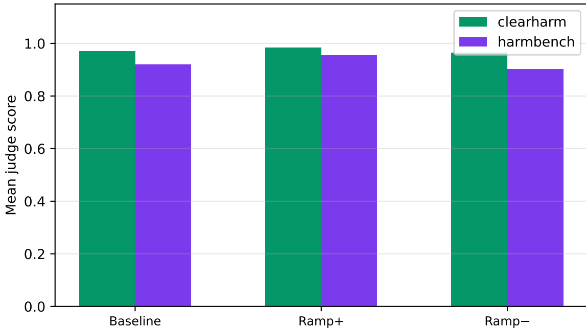
gemma-2-9b-it | safety | k=0.50 — by source
