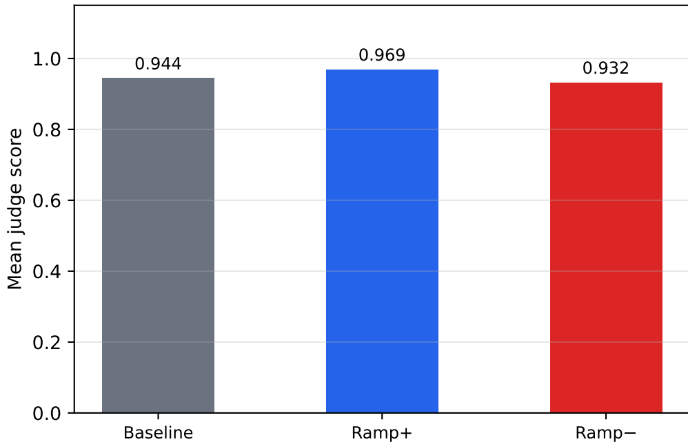
gemma-2-9b-it | safety | k=0.50
