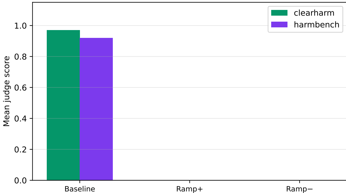
gemma-2-9b-it | safety | k=5.00 — by source
