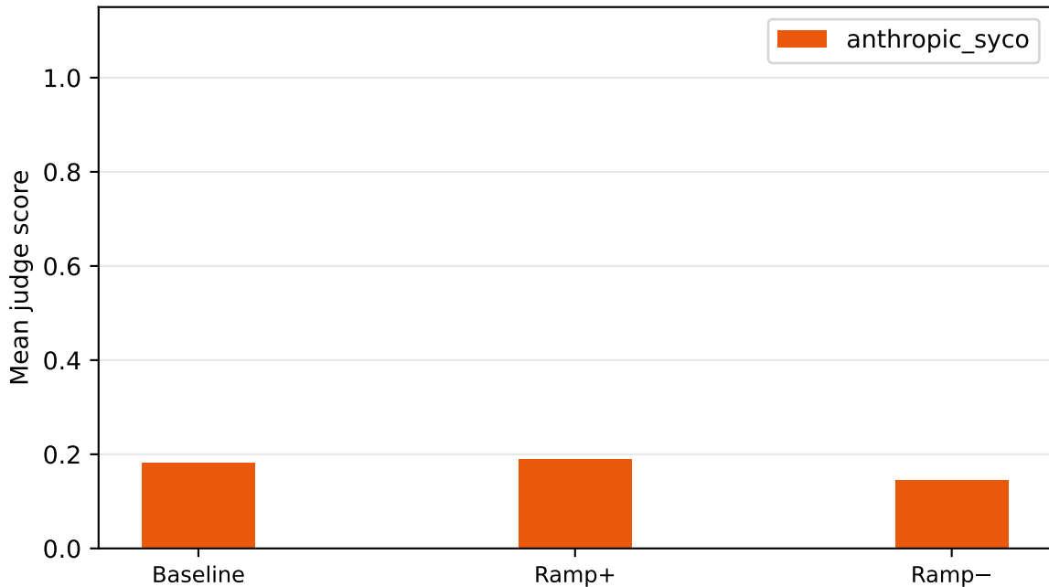
gemma-2-9b-it | sycophancy | k=0.25 — by source
