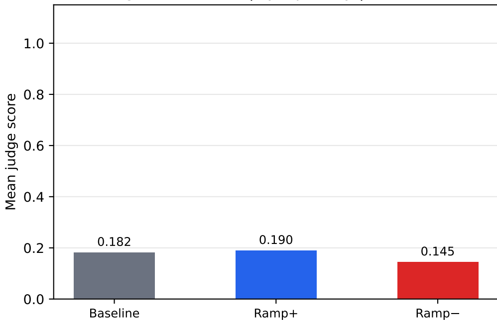
gemma-2-9b-it | sycophancy | k=0.25
