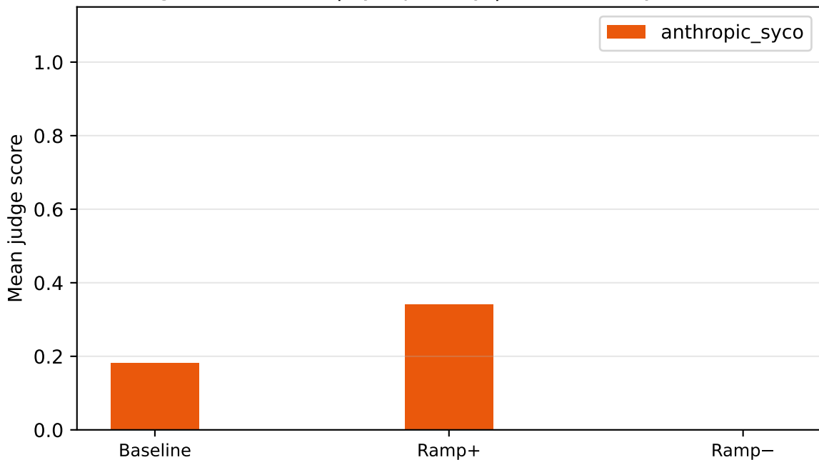
gemma-2-9b-it | sycophancy | k=3.00 — by source
