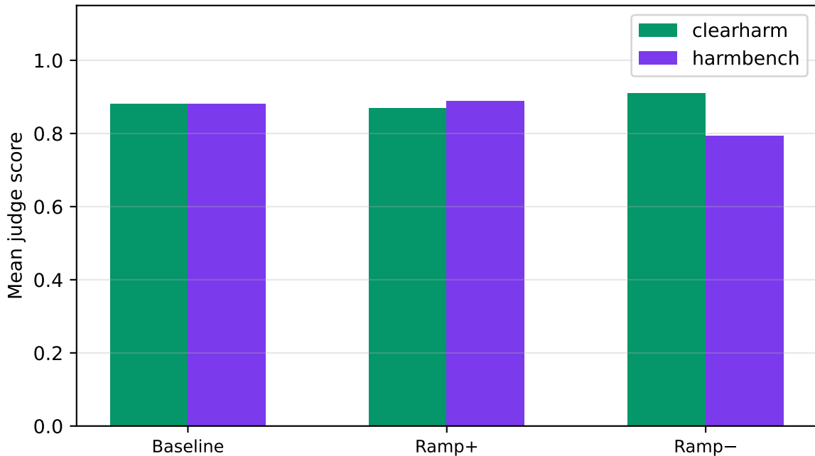
llama-3.1-8b-instruct | safety | k=0.25 — by source
