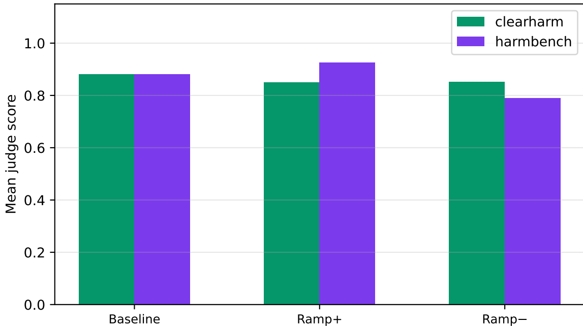
llama-3.1-8b-instruct | safety | k=0.50 — by source
