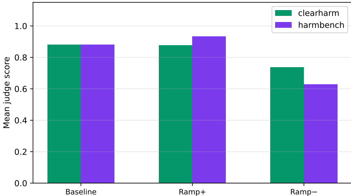
llama-3.1-8b-instruct | safety | k=1.00 — by source
