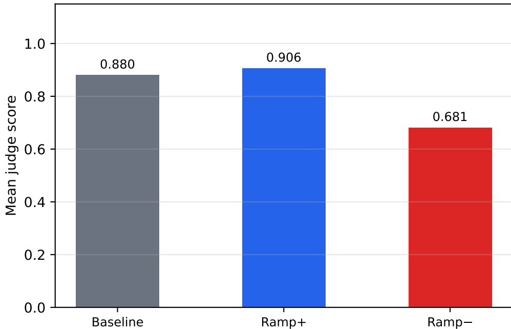
llama-3.1-8b-instruct | safety | k=1.00
