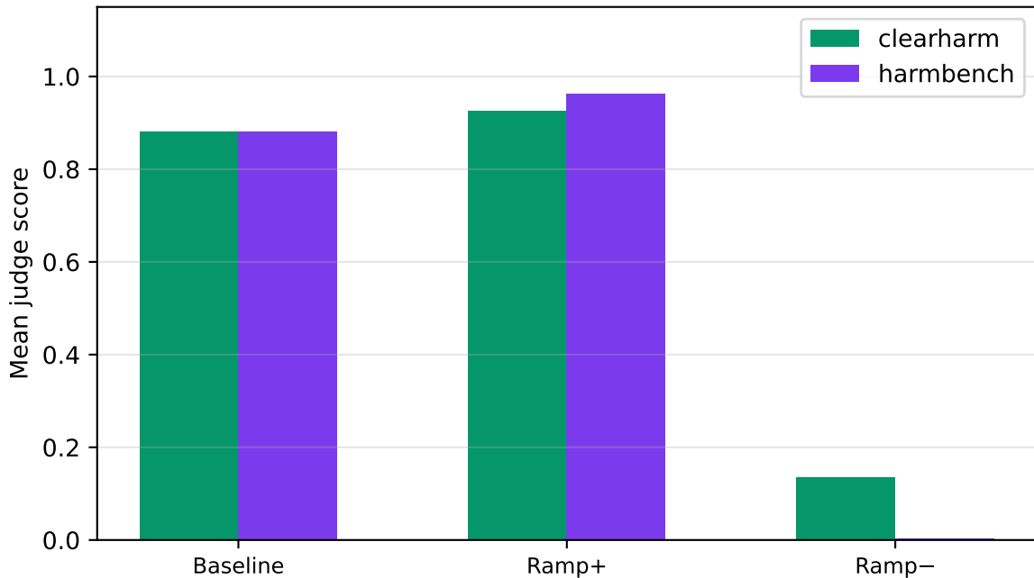
llama-3.1-8b-instruct | safety | k=2.00 — by source
