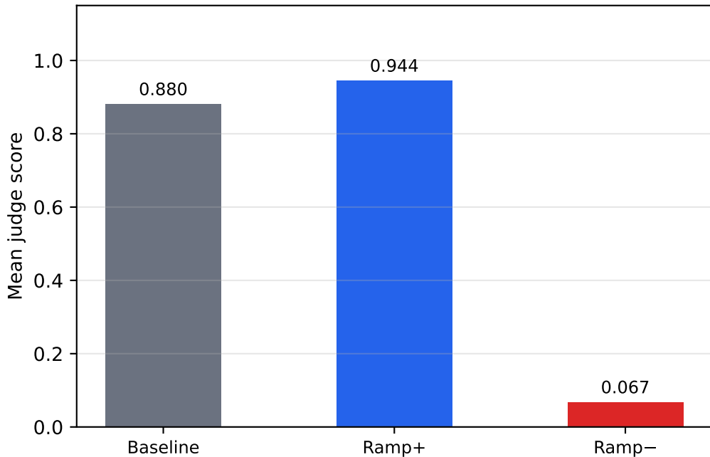
llama-3.1-8b-instruct | safety | k=2.00
