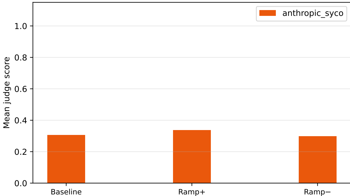
llama-3.1-8b-instruct | sycophancy | k=0.25 — by source
