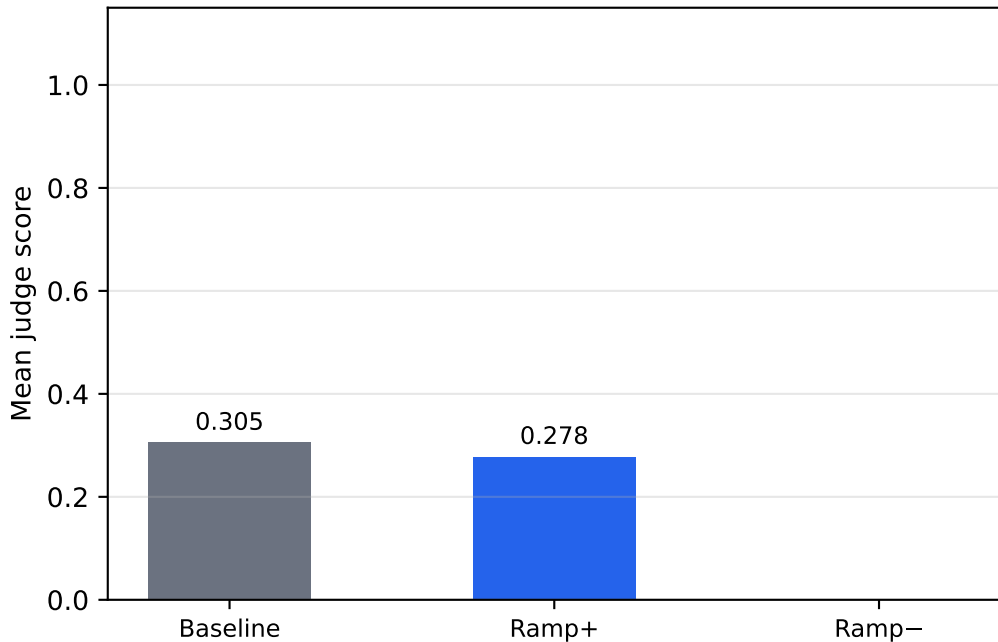
llama-3.1-8b-instruct | sycophancy | k=1.00
