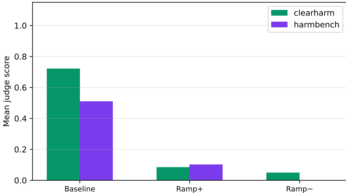
mistral-7b-instruct | safety | k=2.00 — by source
