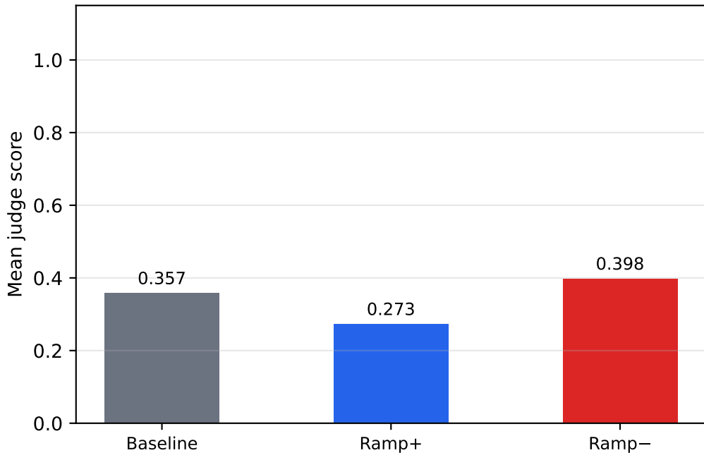
mistral-7b-instruct | sycophancy | k=0.25
