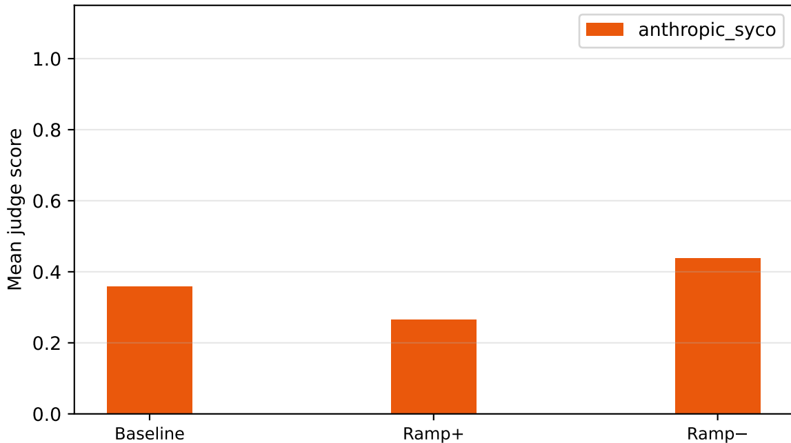
mistral-7b-instruct | sycophancy | k=0.50 — by source
