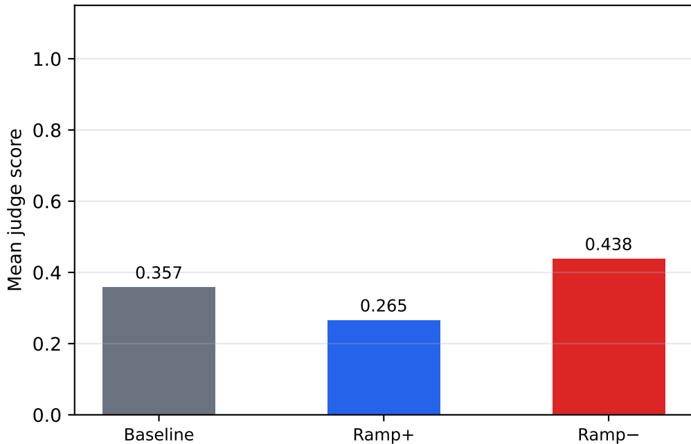
mistral-7b-instruct | sycophancy | k=0.50
