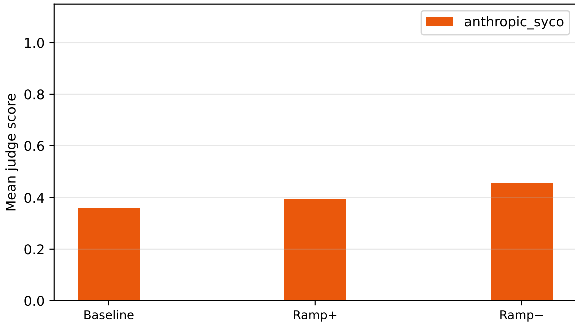
mistral-7b-instruct | sycophancy | k=1.00 — by source
