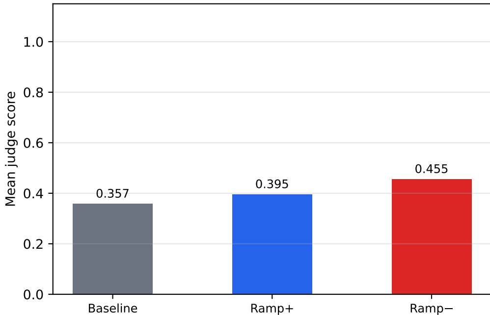
mistral-7b-instruct | sycophancy | k=1.00
