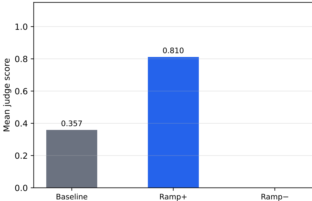
mistral-7b-instruct | sycophancy | k=3.00
