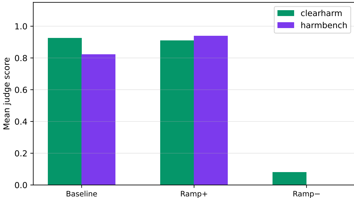
qwen2.5-7b-instruct | safety | k=1.00 — by source
