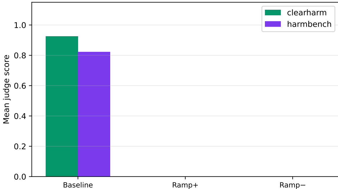
qwen2.5-7b-instruct | safety | k=3.00 — by source
