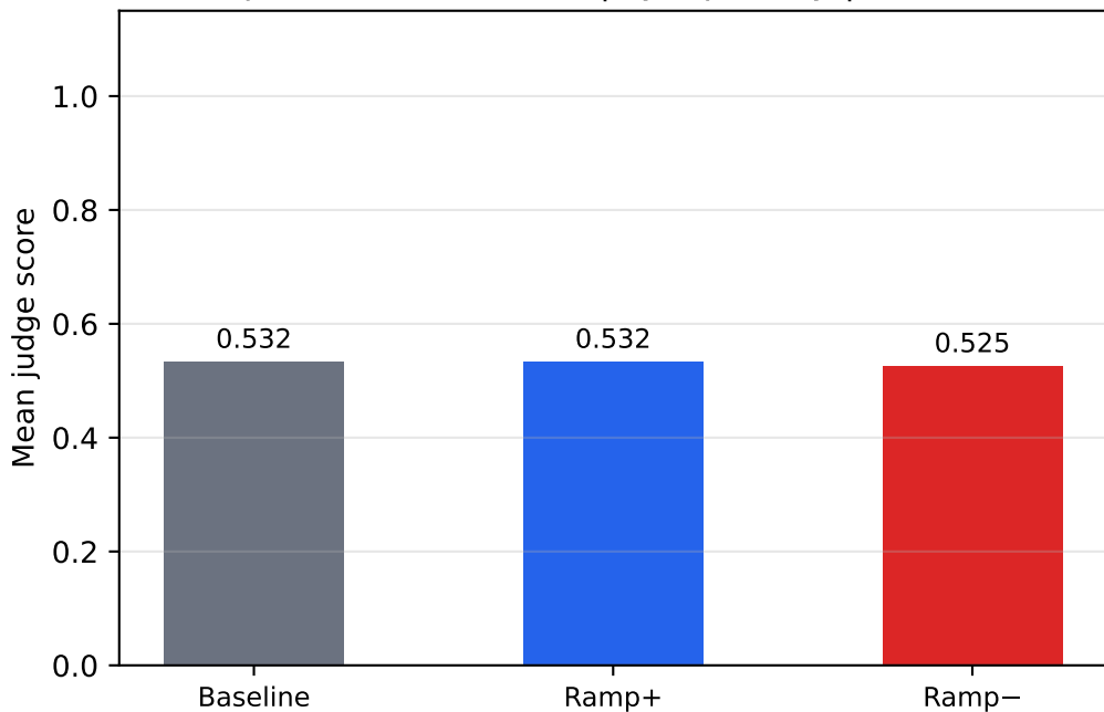
qwen2.5-7b-instruct | sycophancy | k=0.25
