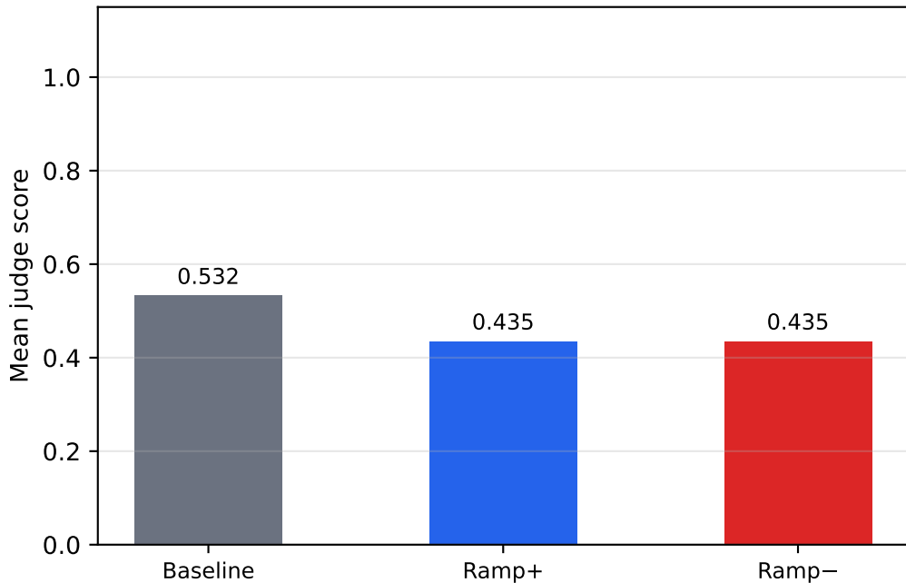
qwen2.5-7b-instruct | sycophancy | k=0.50
