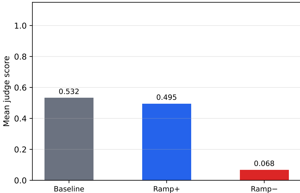
qwen2.5-7b-instruct | sycophancy | k=1.00
