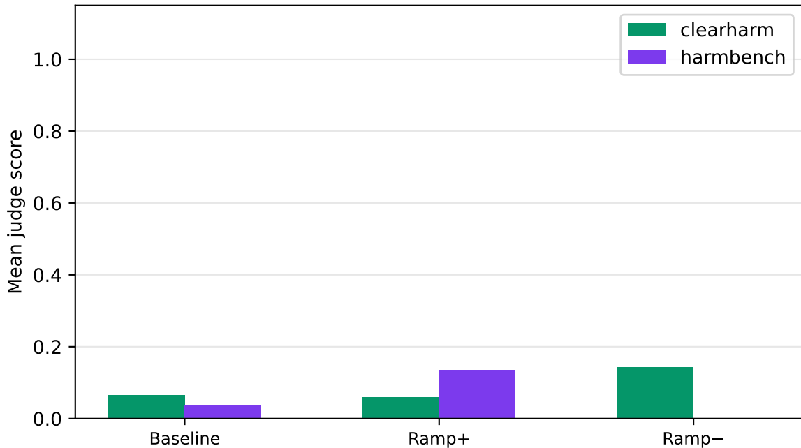
gemma-2-9b | safety | k=0.50 — by source
