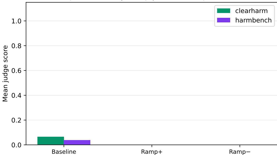
gemma-2-9b | safety | k=3.00 — by source
