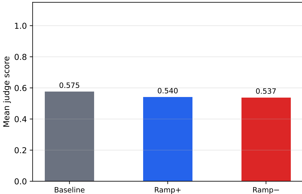
gemma-2-9b | sycophancy | k=0.25
