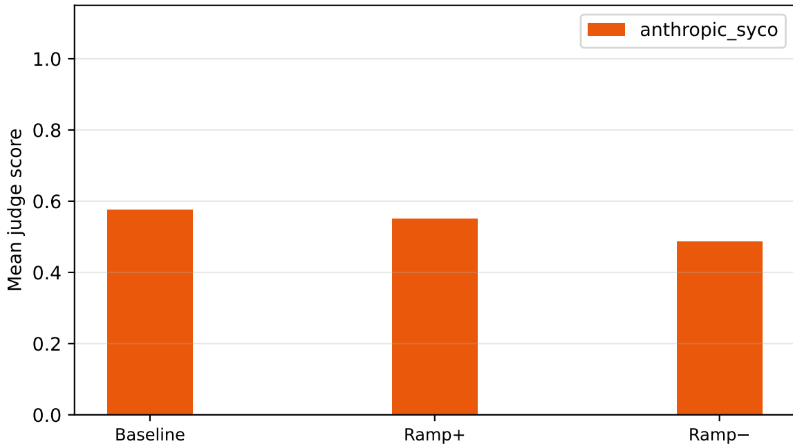
gemma-2-9b | sycophancy | k=0.50 — by source
