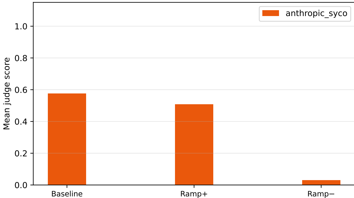
gemma-2-9b | sycophancy | k=2.00 — by source
