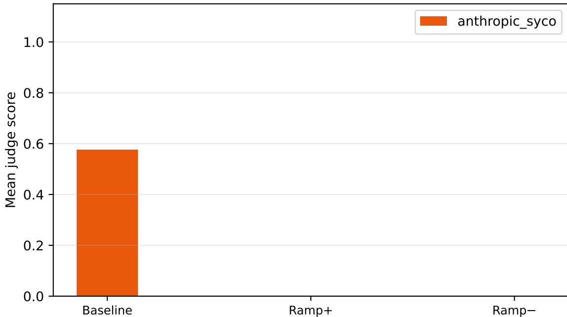
gemma-2-9b | sycophancy | k=5.00 — by source
